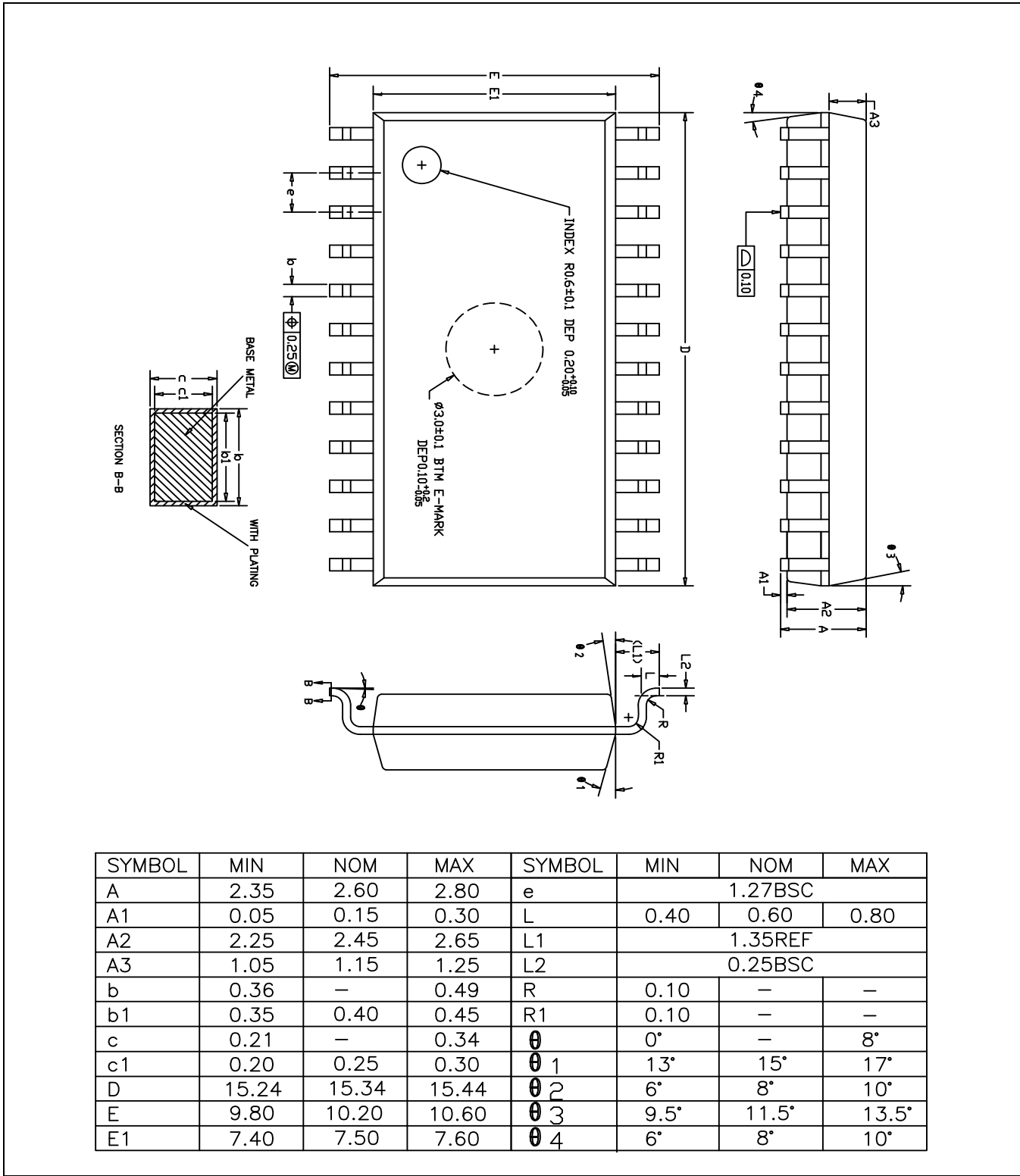
Figure 4-2 SOP24 (1.27mm)封装尺寸
